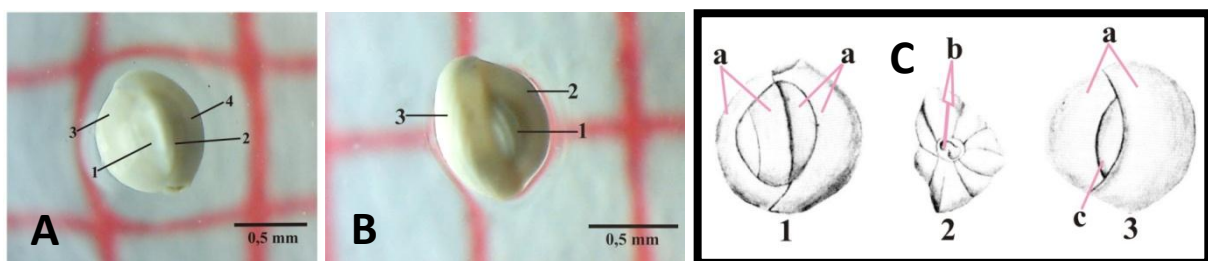
Gambar 2. Quinqueloculina lamarckiana ; A. tampak depan, 4 kamar (1-4), B. tampak belakang, 3 kamar (1-3) C. Sketsa (sumber: Ellis dan Messina, 1959): 1. Tampak depan, 4 kamar (a. kamar); 2. Tampak atas (b. aperture); 3. Tampak belakang, 3 kamar (a. kamar, c. proloculus).
